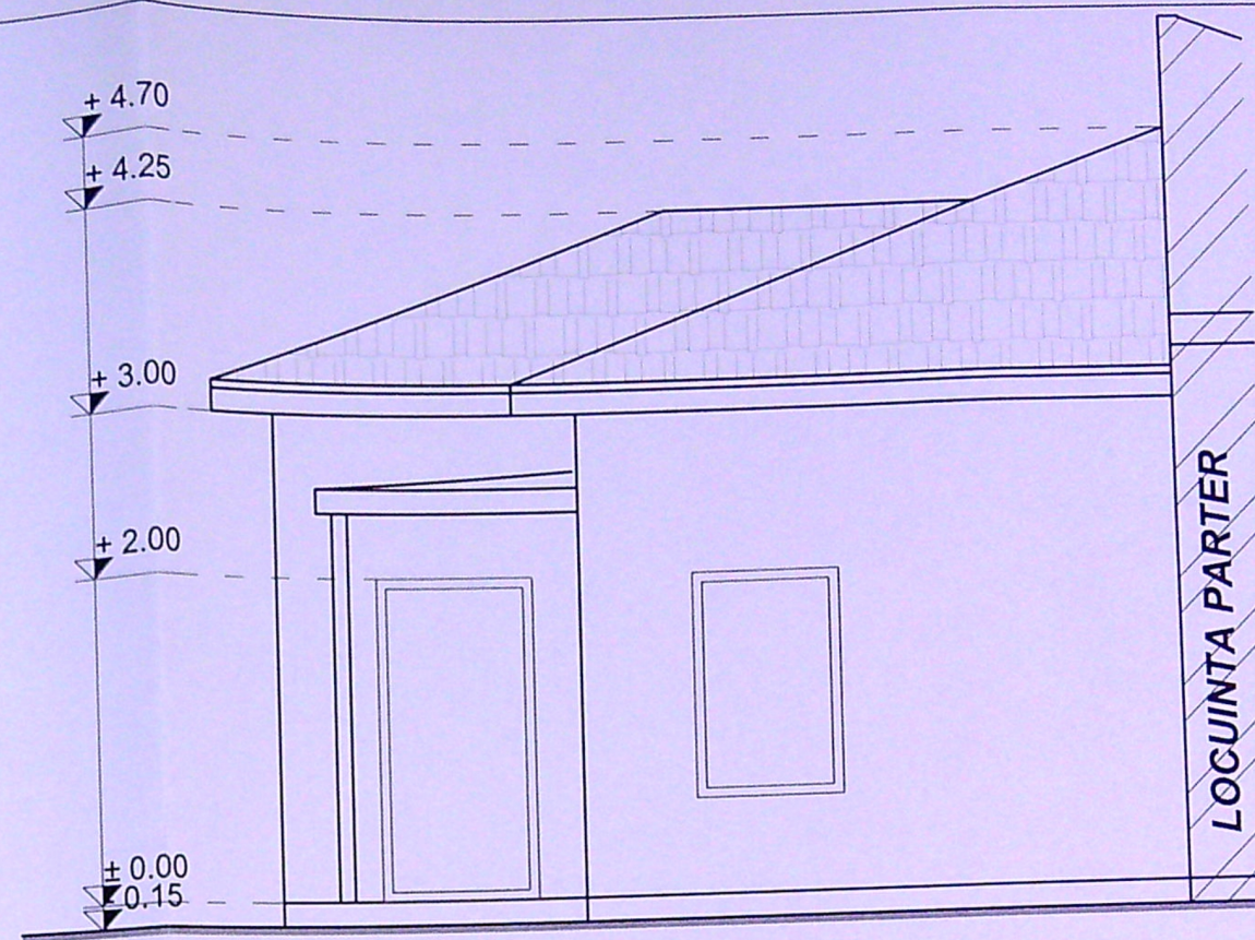
FATADA PRINCIPALA
